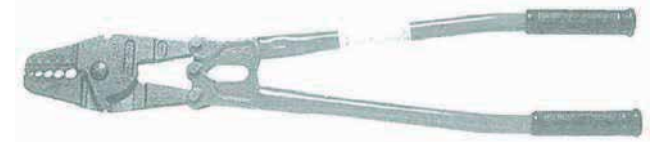
Model hsc - 350 swages 2mm to 3,5 rope Model hsc - 600 swages 2mm to 5mm rope
