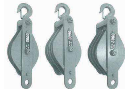
Wire Rope Reeving Blocks
